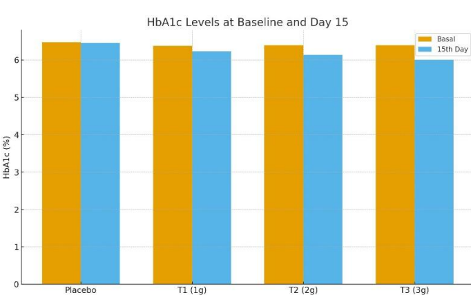
Figure 2 HbA1c levels at Baseline and Day 15
