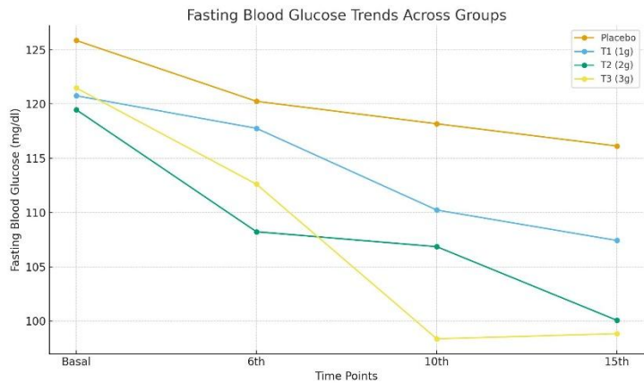
Figure 2 Fasting Blood glucose Trends Across Groups
